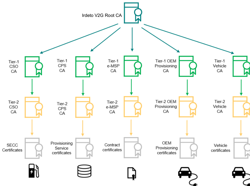
Figure 1: Overview of the Irdeto CrossCharge V2G PKI for ISO 15118-20
